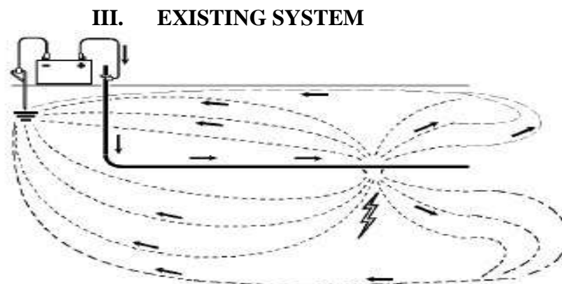
Figure 1 An A-Frame method of finding cable fault location
