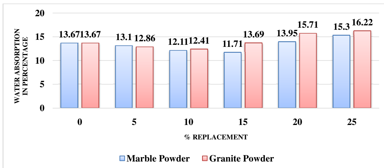
Figure 3: Water absorption v/s % Marble Powder and Granite Powder
