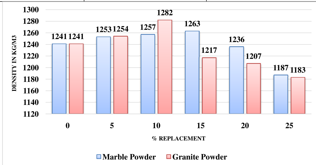
Figure 2: Density v/s % Marble Powder and Granite Powder
