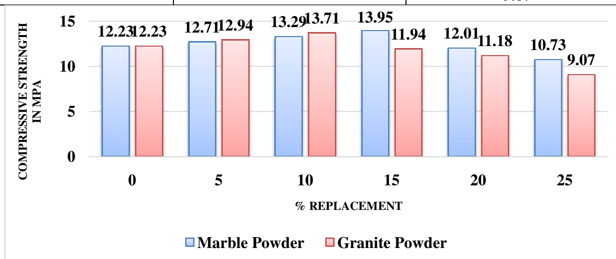
Figure 1: Compressive strength v/s % Marble Powder and Granite Powder
