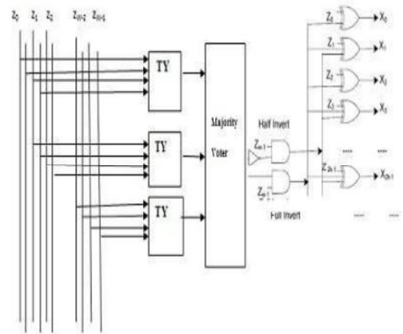
Fig.4. Decoder architecture scheme II
