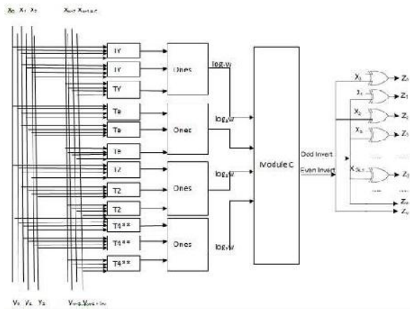
Fig.5. Encoder architecture for scheme III
