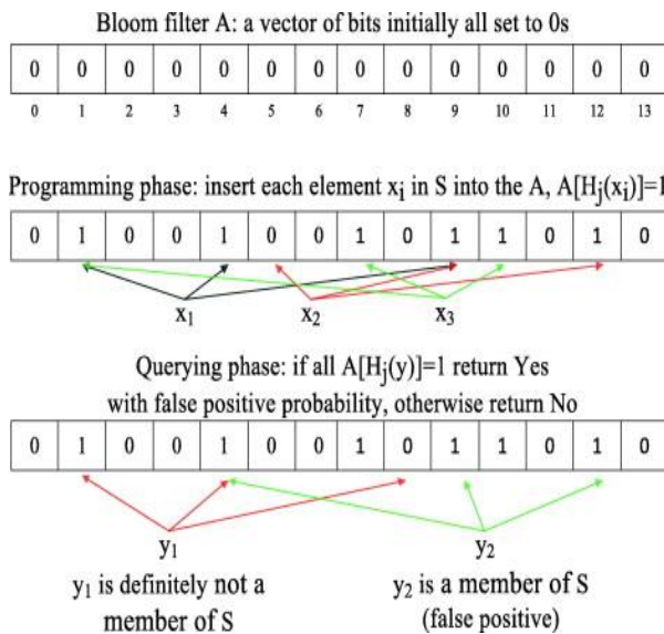
Fig1. Counting bloom filter process
