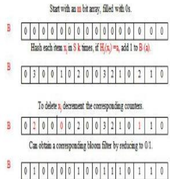
Fig2. Example of Counting bloom filter process
