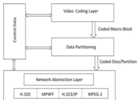
Figure 2. Structure of H.264/AVC Video Encoder
