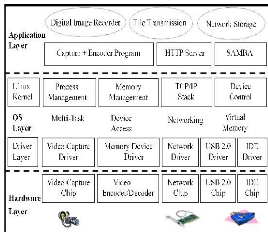
Figure 1. System architecture
