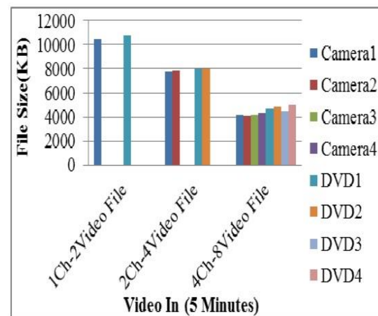
Figure 12. File size of 5 minute video recorded in USB flash drive of a Nuvoton ARM9-NUC960 embedded system
