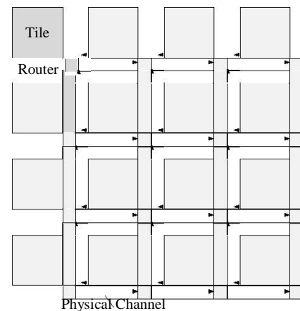
Figure 1. On-Chip Network. Each tile may contain identical logic, as in the case of a multiprocessor or tiled system, or simply represent a partitioning of a SoC design.
