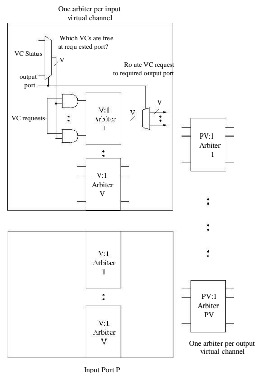
Figure 3. Arbitration complexity of a virtual channel allocator. In this example, the routing function returns a single output port and one or more VC requests.
