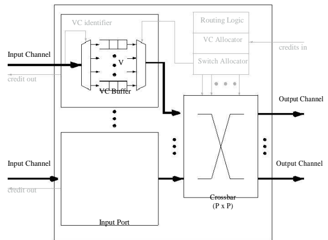
Figure 2. Virtual-Channel Router
