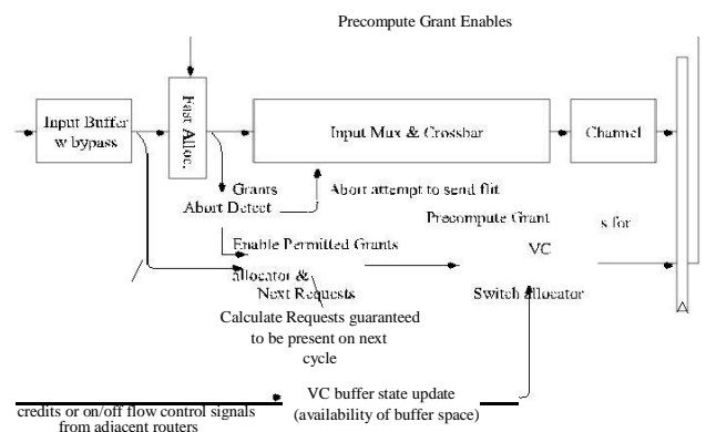
Figure 7. Data dependencies within our single-cycle optimised router architecture
