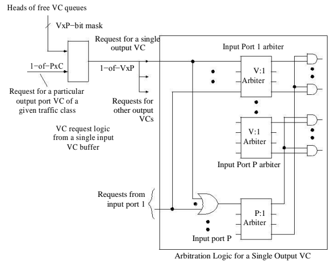
Figure 5. Virtual Channel Allocator logic. A free VC queue and tree arbiter organisation is used to simplify the implementation.
