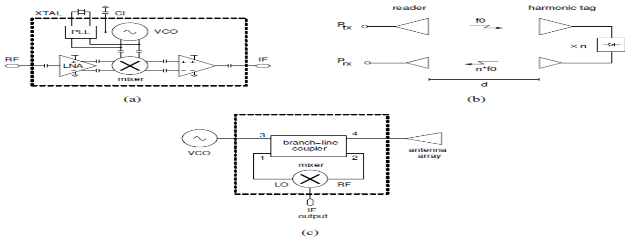
Figure 1. Architecture of three typical communication and wireless sensing systems, namely: (a) super-heterodyne receiver; (b) harmonic RFID tag; (c) Doppler radar sensor. The main building blocks involved are antennas, amplifiers, oscillators, mixers and frequency multipliers.
