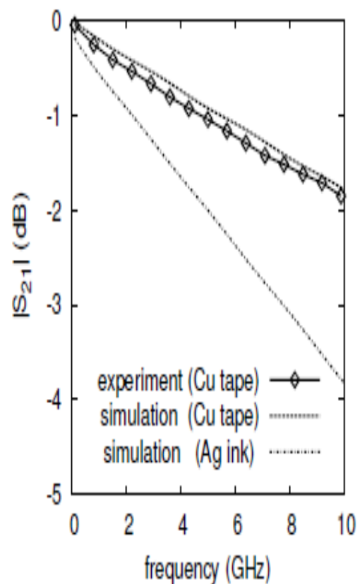
Figure 3. Transmission parameter S_{21} of a 50 \Omega , copper microstrip line versus the frequency. The track is 30 mm long and is compared with a similar structure made out of Ag ink ( 3 \mu\text{m} ink thickness, \sigma_{ink} = 1.1 \times 10^7 \text{ S/m} after curing). Reproduced with permission from [12]. Copyright 2012, IEEE.
