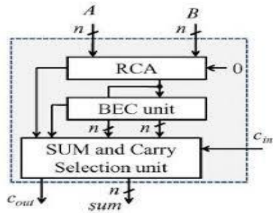
Figure 3. BEC Based CSLA
