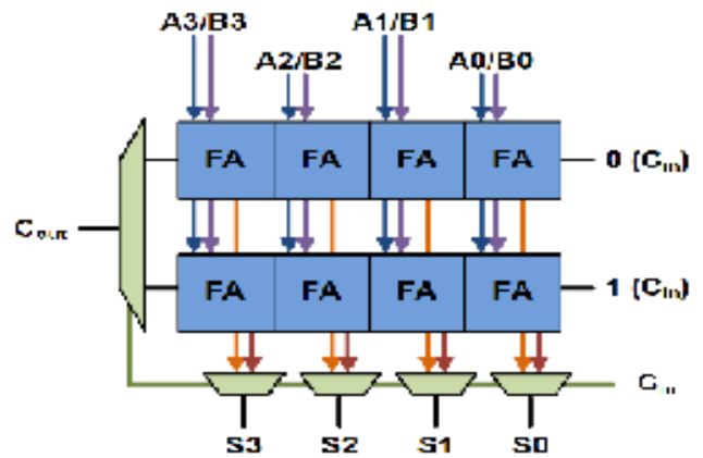
Figure 1 Carry Select Adder.
