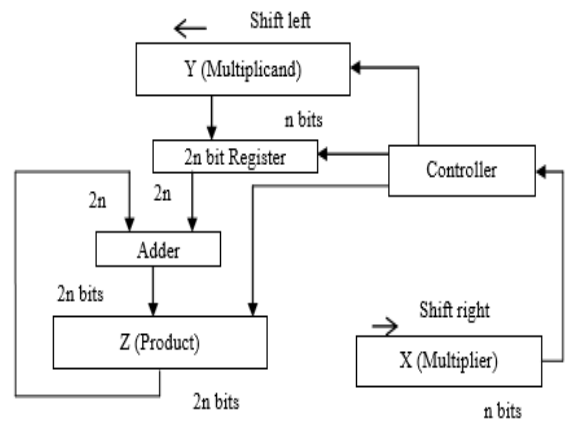
Figure 5. Multiplication Process Schematic
