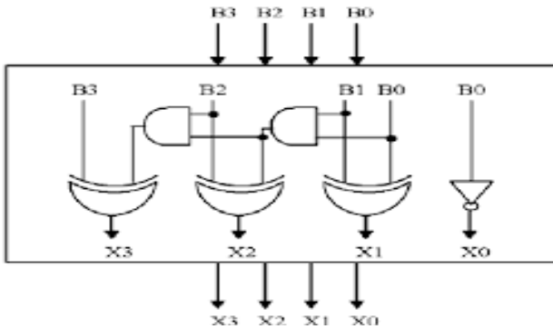
Figure 2. 4-bit Binary to Excess One Converter
