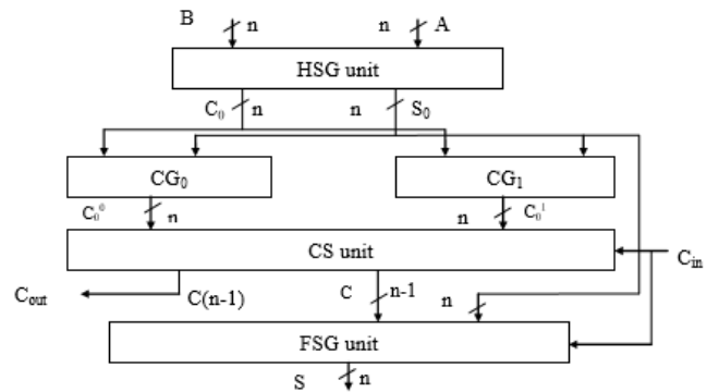
Figure 4. The New Logic Formulation CSLA
