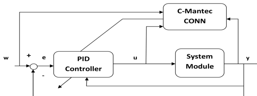
Figure 2. Structure of the C-Mantec CONN using PID Controller.
