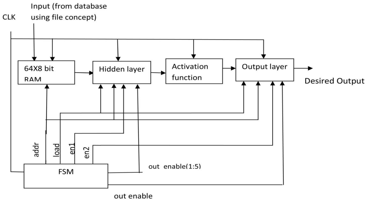
Figure 3. Neural network model.
