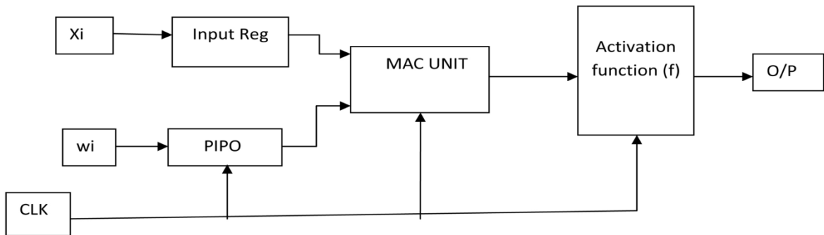
Figure 5. VHDL design of single neuron.
