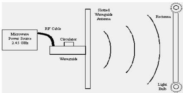
Fig.2 shows Block diagram for wireless energy transfer
