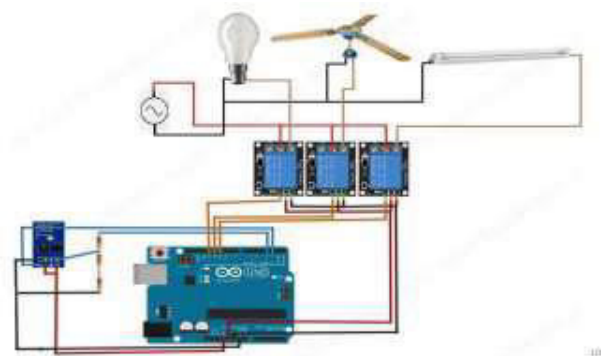
Figure 9: Power circuit
